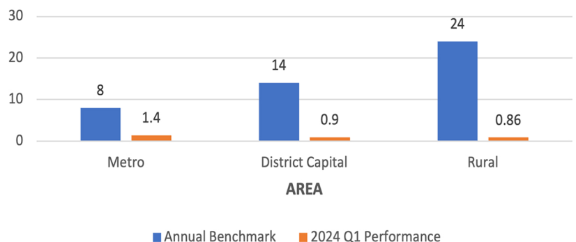
CAIDI (Hours/Customer)
