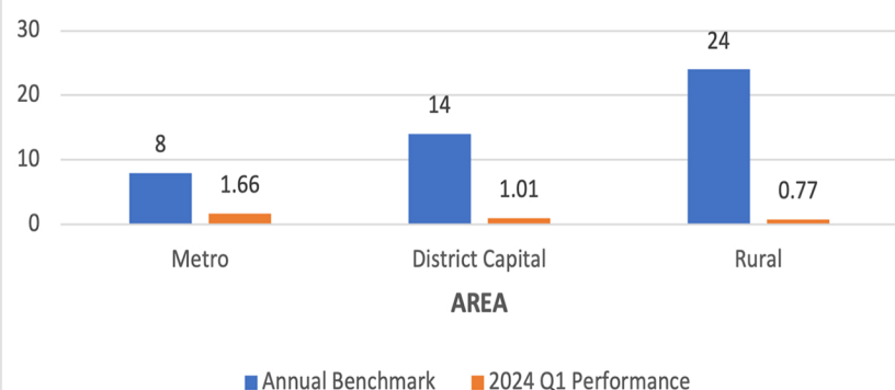
CAIDI (Hours/Customer)
