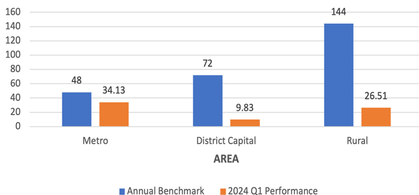
SAIDI (Hours/Customer)
