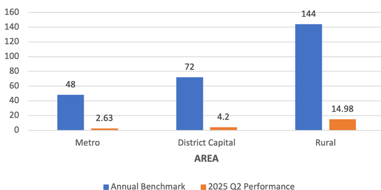
SAIDI (Hours/Customer)
