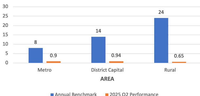
CAIDI (Hours/Customer)
