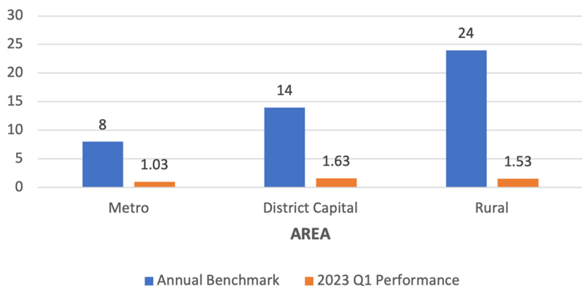
CAIDI (Hours/Customer)
