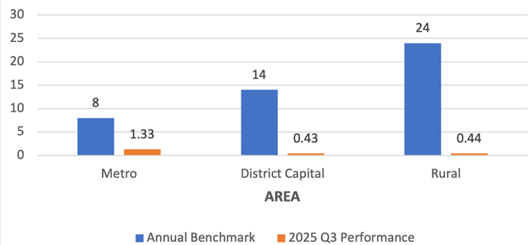
CAIDI (Hours/Customer)
