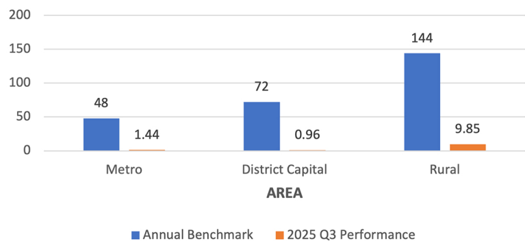
SAIDI (Hours/Customer)
