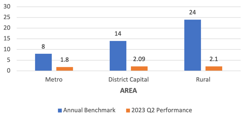
CAIDI (Hours/Customer)
