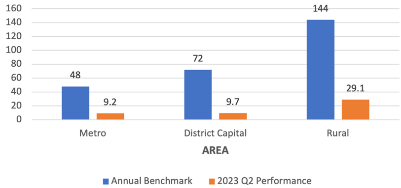
SAIDI (Hours/Customer)
