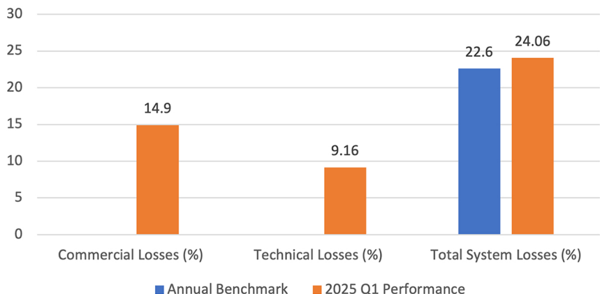
SYSTEM LOSSES
